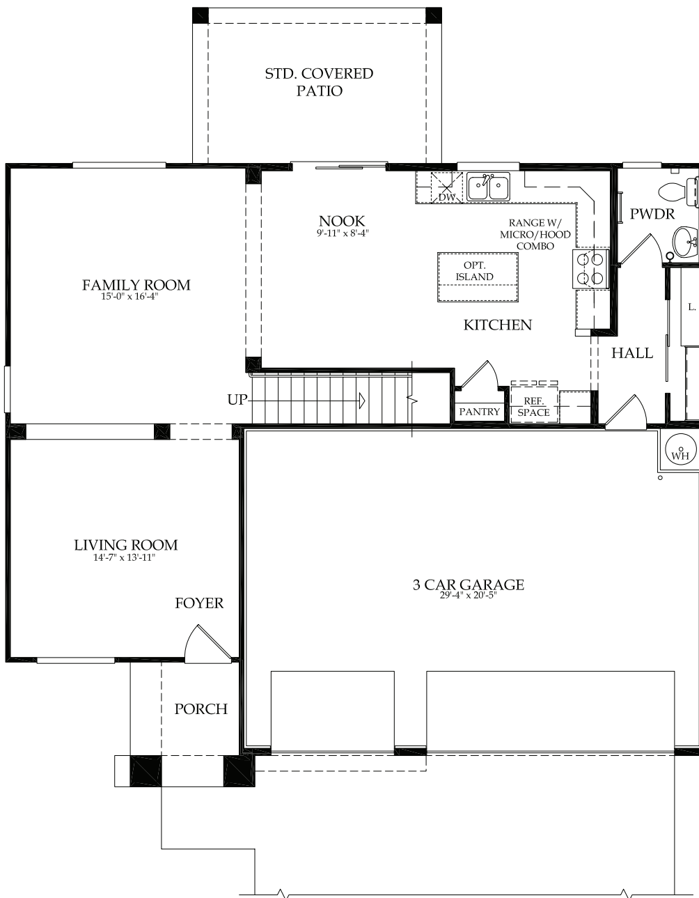
First Floor Plan Elevation A
