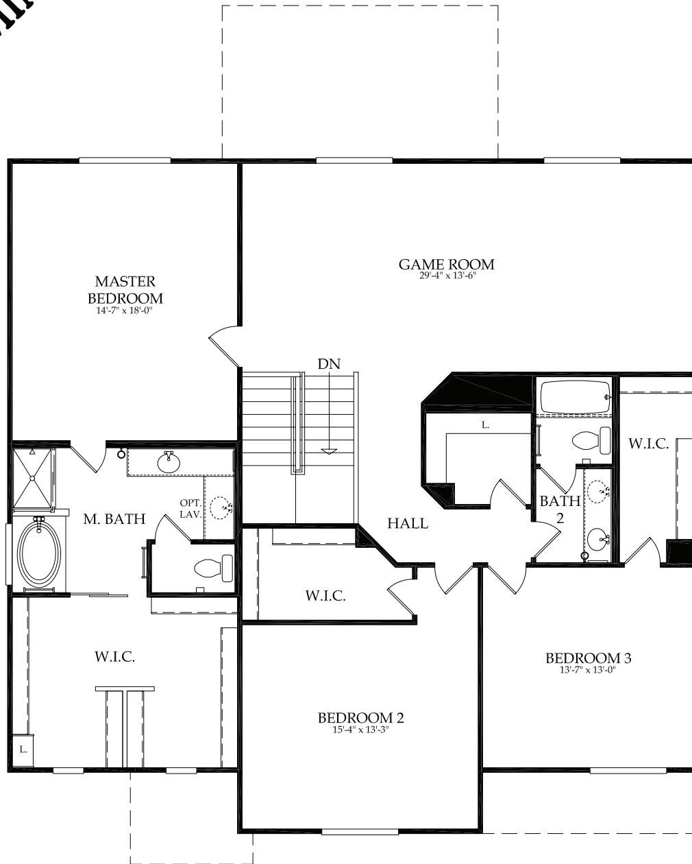
Second Floor Plan Elevation A
