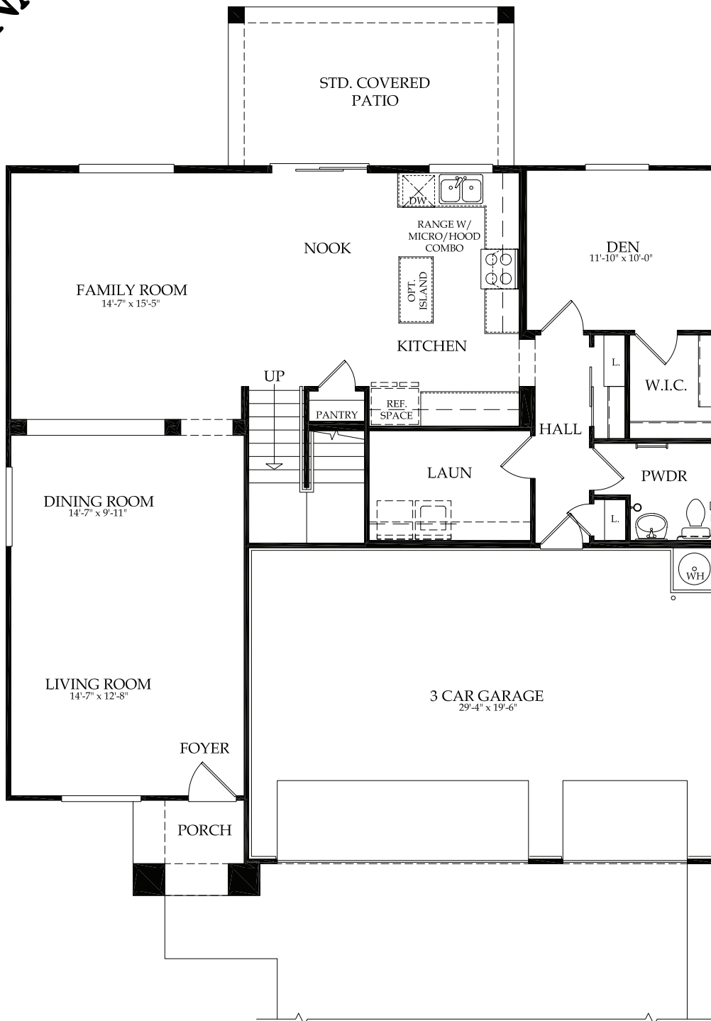
First Floor Plan Elevation A
