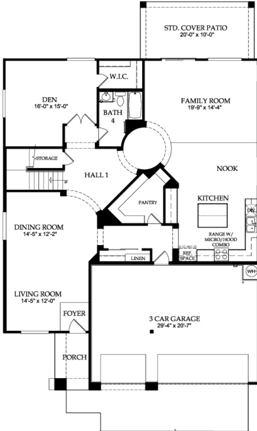
FIRST FLOOR PLAN ELEVATION A
