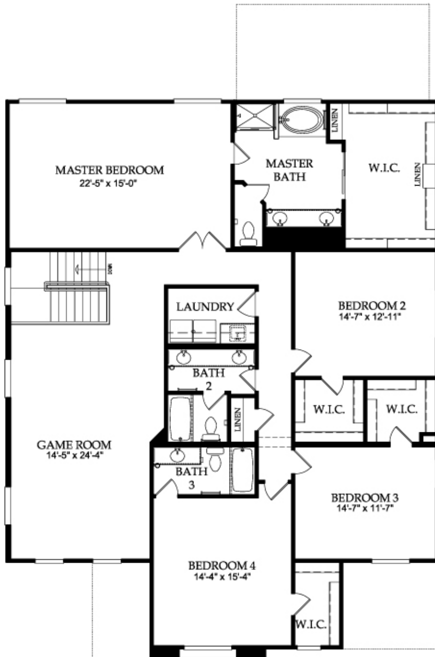
SECOND FLOOR PLAN ELEVATION A
