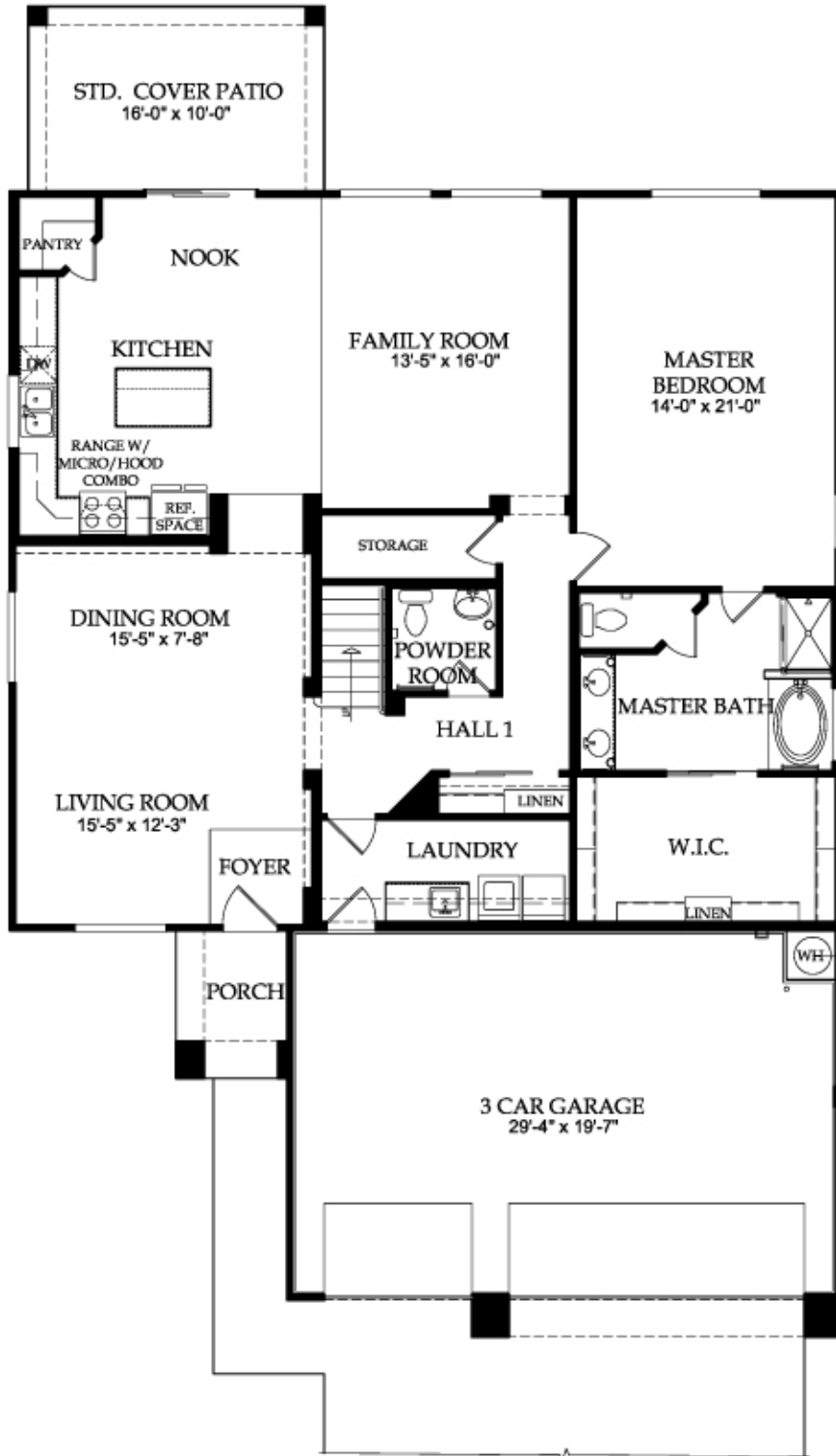
FIRST FLOOR PLAN ELEVATION A
